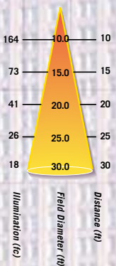
Flood Focus with 150w CDM150/T6 Lamp 85 CRI
