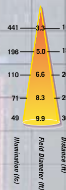
Spot Focus with 150w CDM150/T6 Lamp 85 CRI
